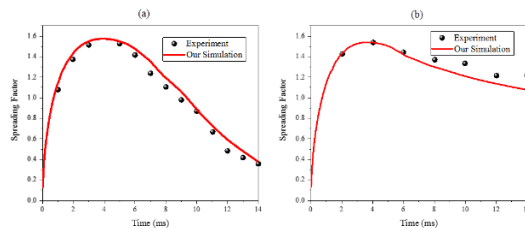
Figure 4: Quantitative comparison of (a) an isothermal and (b) a supercooled droplet impact between the experimental observations by [44] and the present numerical results.
